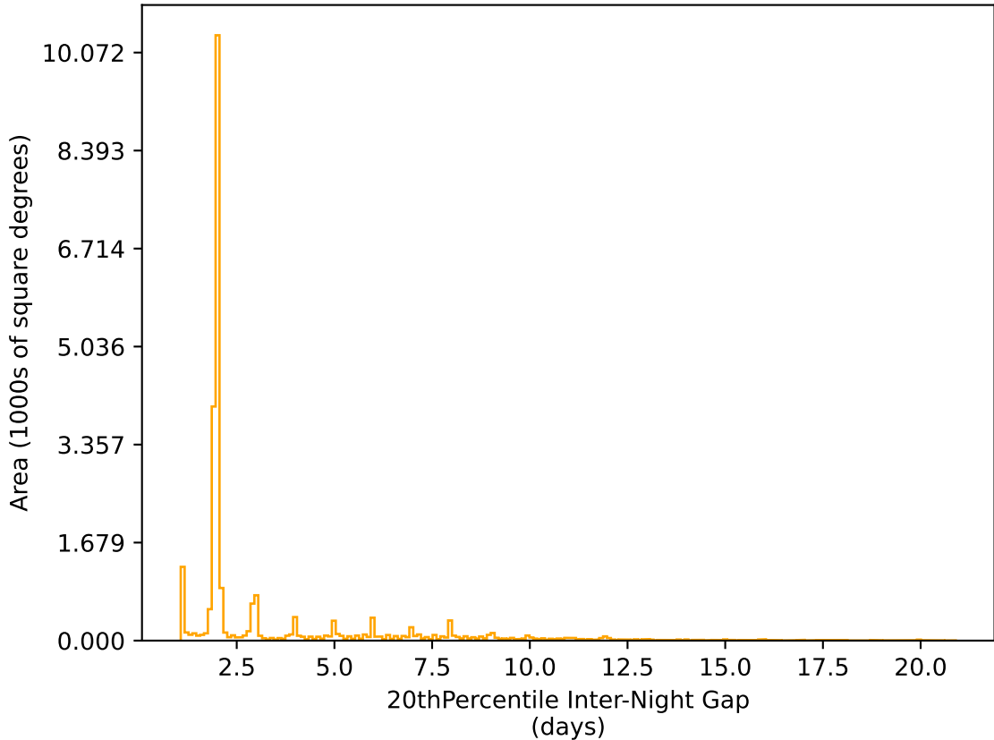
too_elab_r8_d2_gz_v3.4_10yrs All sky r band: 20thPercentile Inter-Night Gap
