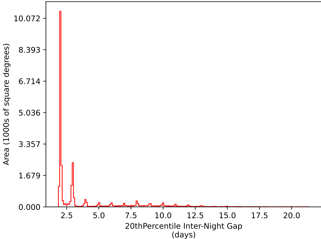
too_elab_r8_d2_gz_v3.4_10yrs All sky i band: 20thPercentile Inter-Night Gap
