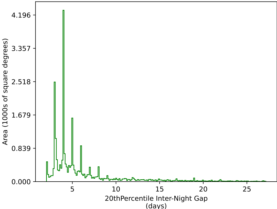
too_elab_r8_d2_gz_v3.4_10yrs All sky g band: 20thPercentile Inter-Night Gap
