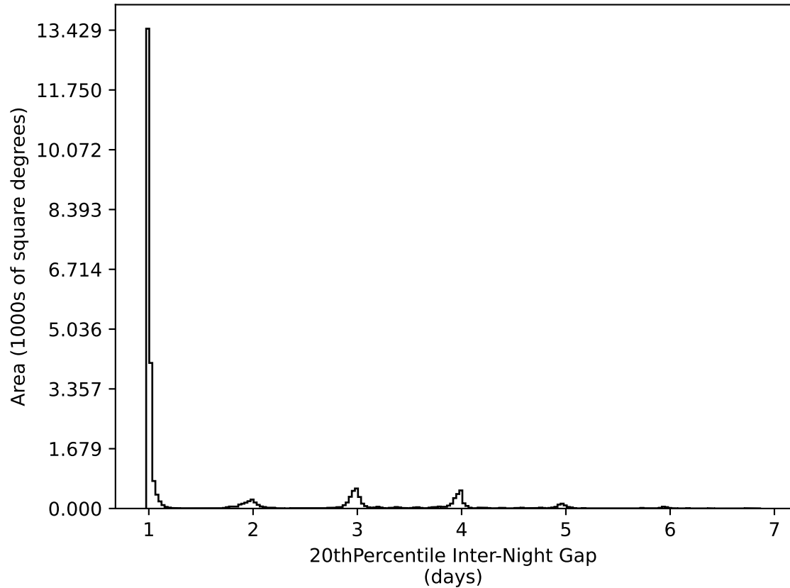
too_elab_r8_d2_gz_v3.4_10yrs All sky all bands: 20thPercentile Inter-Night Gap
