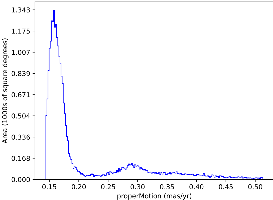
too_elab_r8_d2_gz_v3.4_10yrs : properMotion
