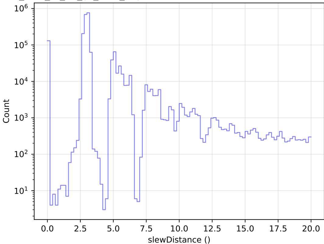
too_elab_r8_d2_gz_v3.4_10yrs All visits: Zoom Slew Distance Histogram
