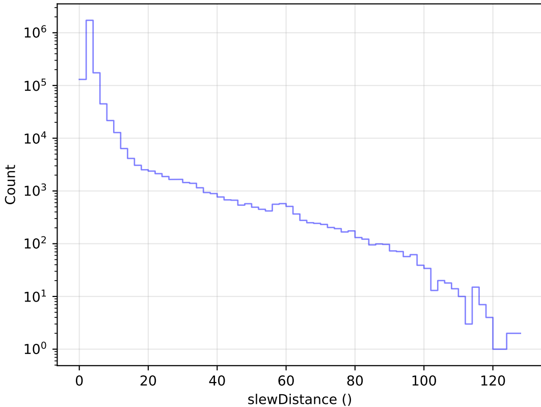
too_elab_r8_d2_gz_v3.4_10yrs All visits: Slew Distance Histogram
