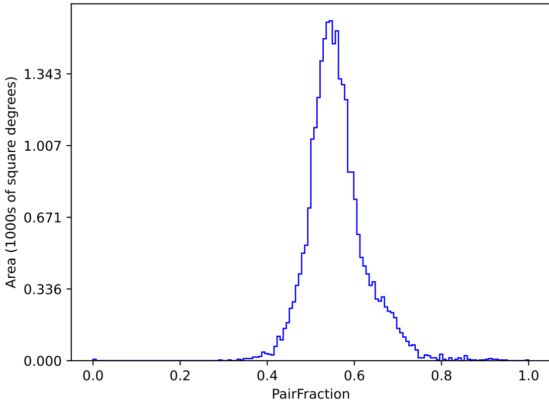
too_elab_r8_d2_gz_v3.4_10yrs (g or r or i): PairFraction
