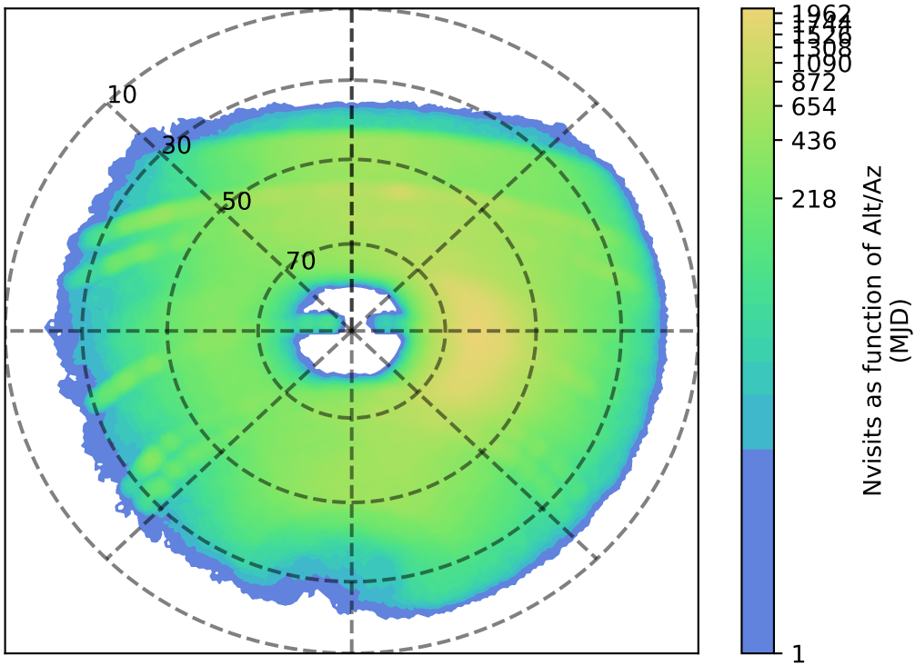
too_elab_r8_d2_gz_v3.4_10yrs y: Nvisits as function of Alt/Az
