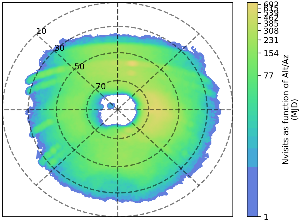
too_elab_r8_d2_gz_v3.4_10yrs u: Nvisits as function of Alt/Az
