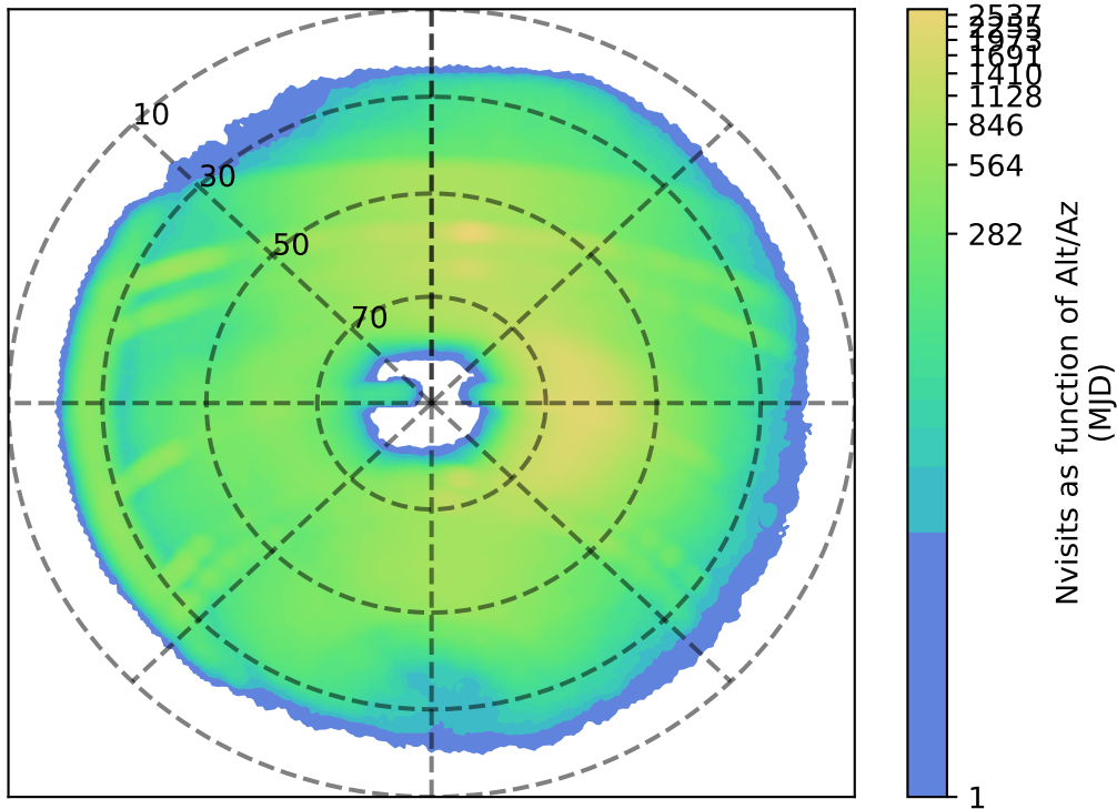
too_elab_r8_d2_gz_v3.4_10yrs r: Nvisits as function of Alt/Az
