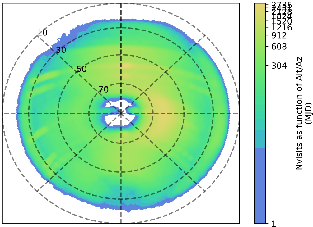
too_elab_r8_d2_gz_v3.4_10yrs i: Nvisits as function of Alt/Az
