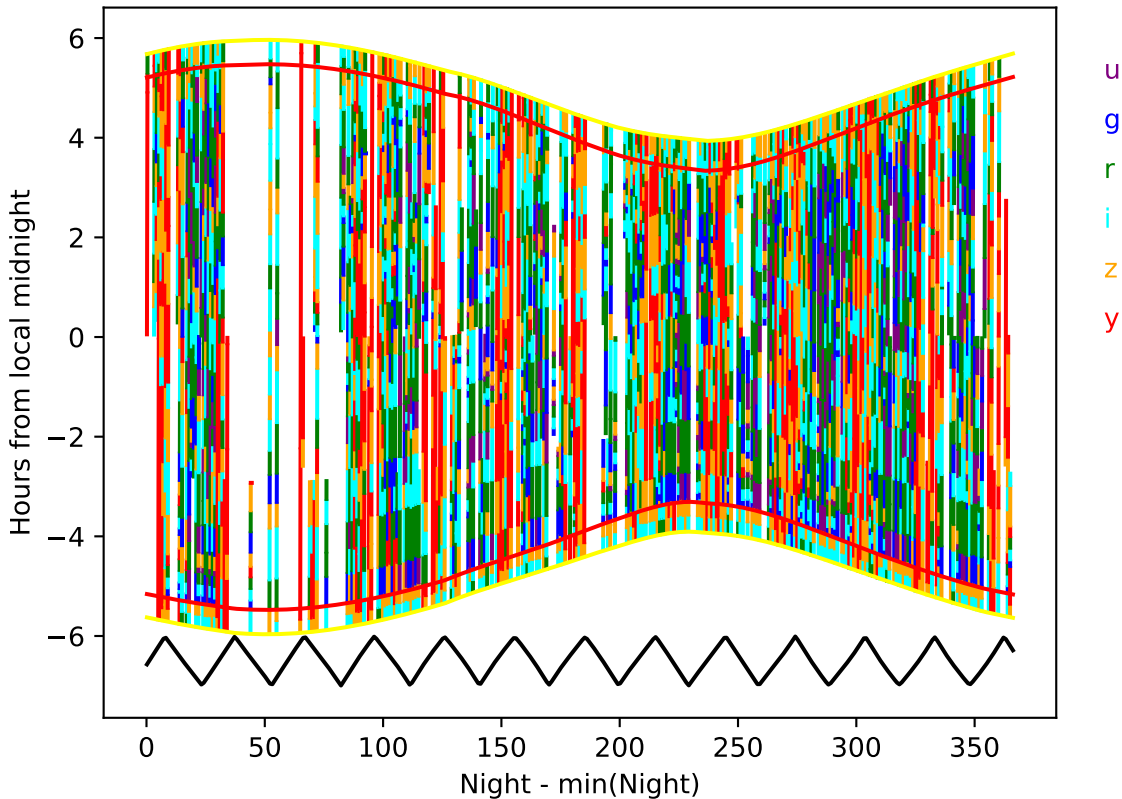
too_elab_r8_d2_gz_v3.4_10yrs year 3-4: Hourglass
