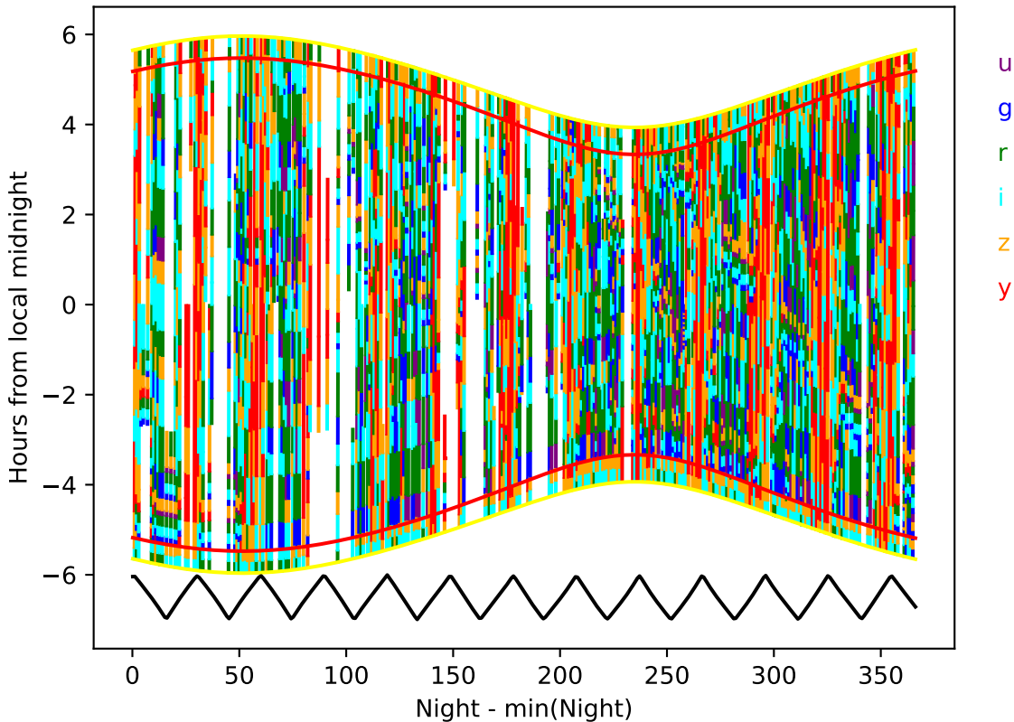
too_elab_r8_d2_gz_v3.4_10yrs year 1-2: Hourglass
