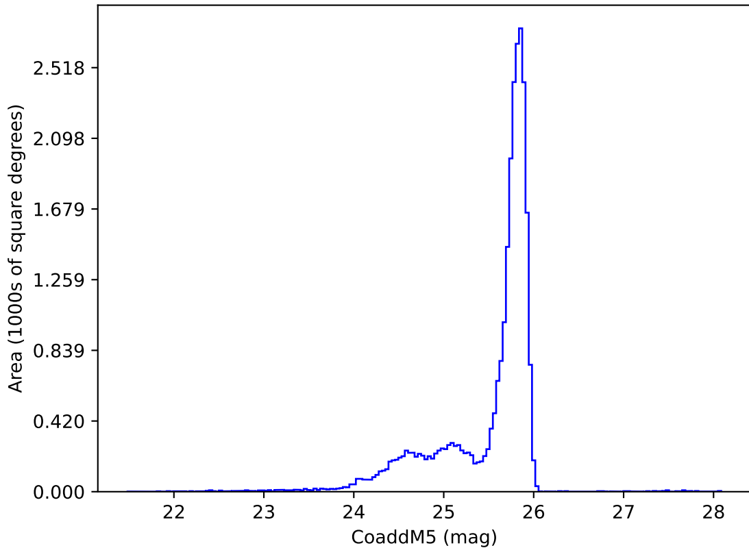
too_elab_r8_d2_gz_v3.4_10yrs z: CoaddM5
