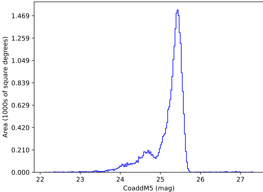
too_elab_r8_d2_gz_v3.4_10yrs u: CoaddM5
