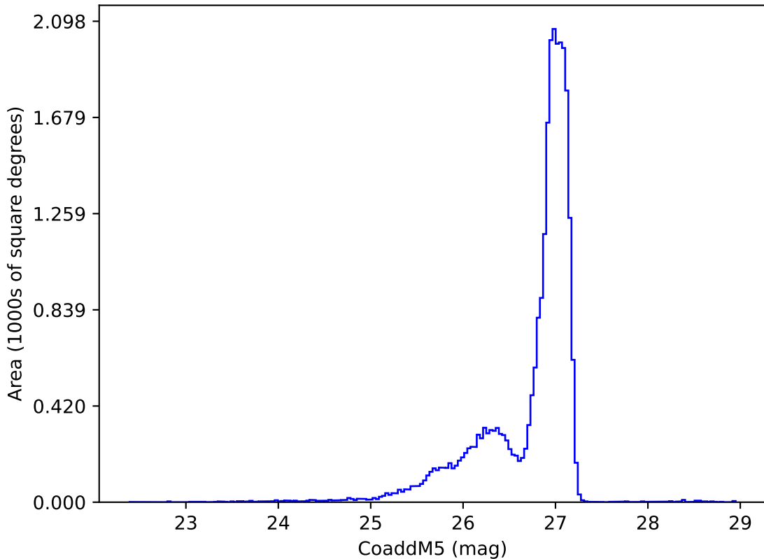
too_elab_r8_d2_gz_v3.4_10yrs r: CoaddM5
