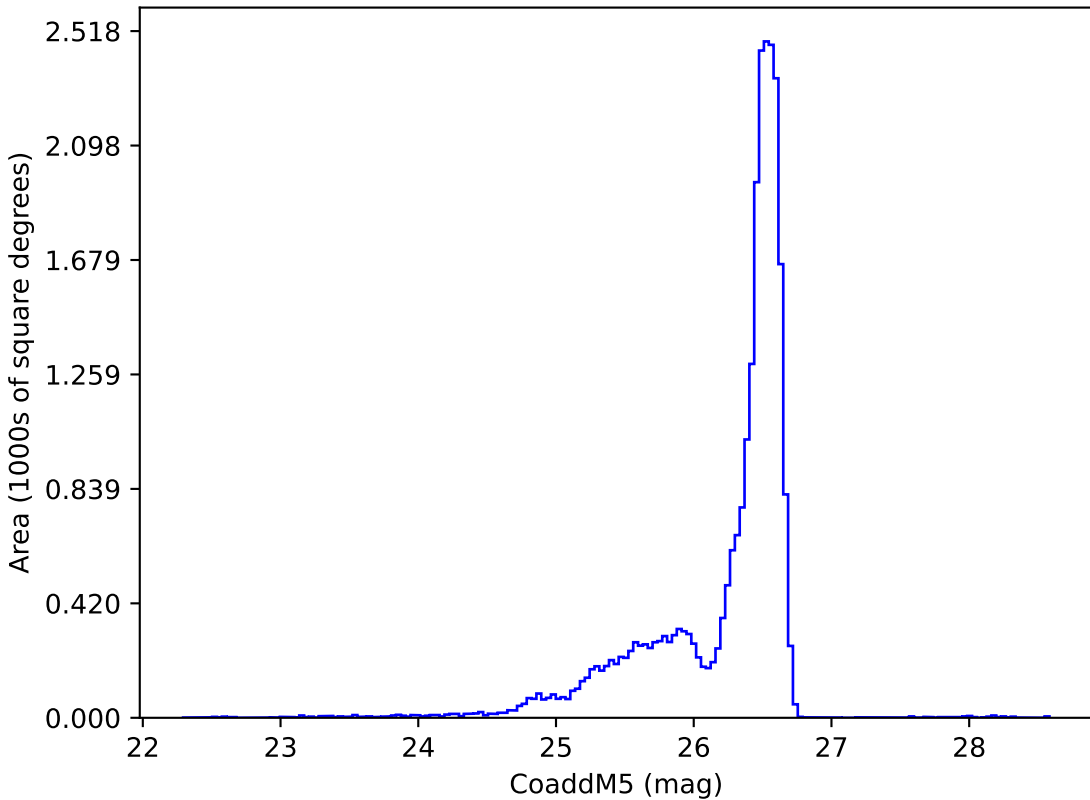
too_elab_r8_d2_gz_v3.4_10yrs i: CoaddM5
