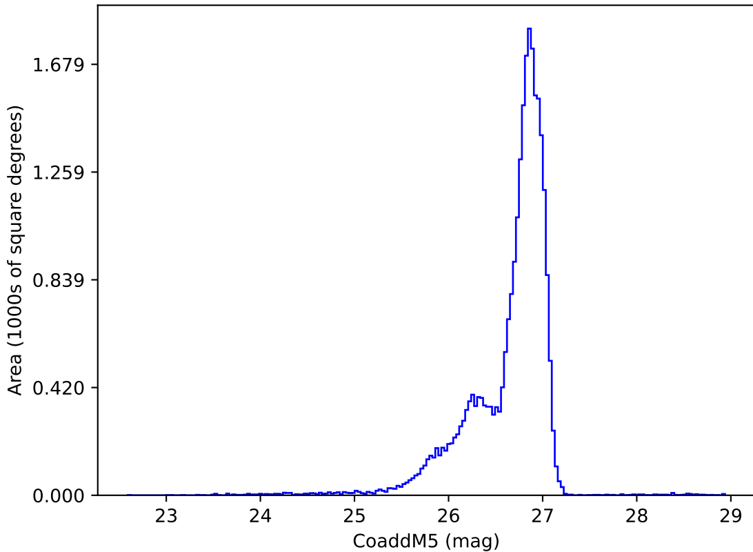
too_elab_r8_d2_gz_v3.4_10yrs g: CoaddM5
