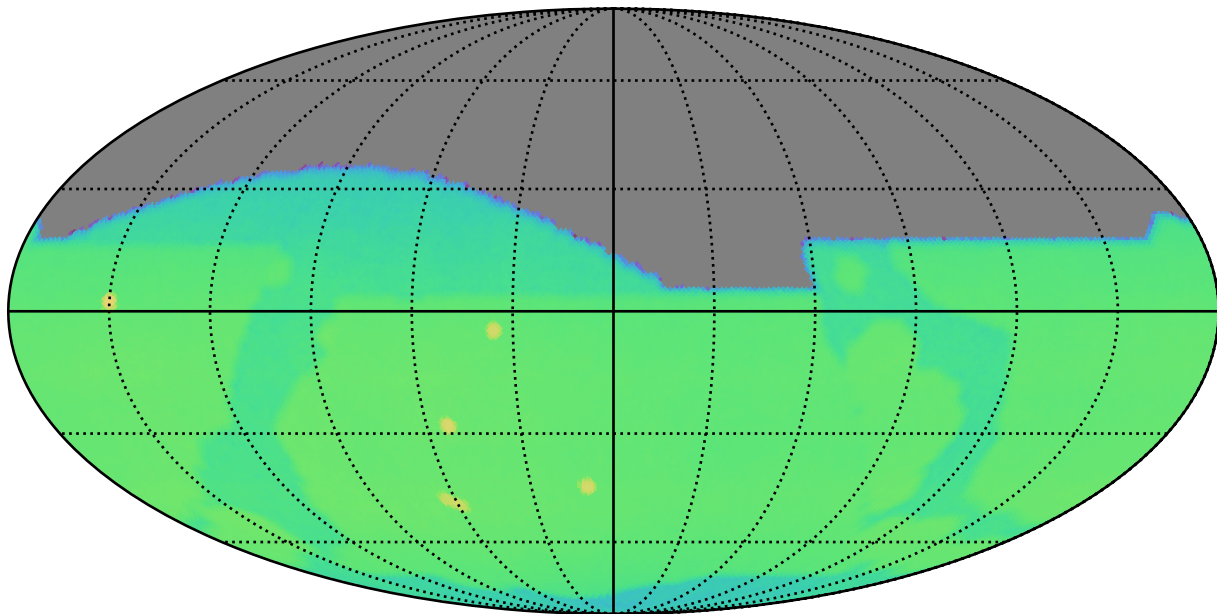
too_elab_r8_d2_gz_v3.4_10yrs : CoaddM5
