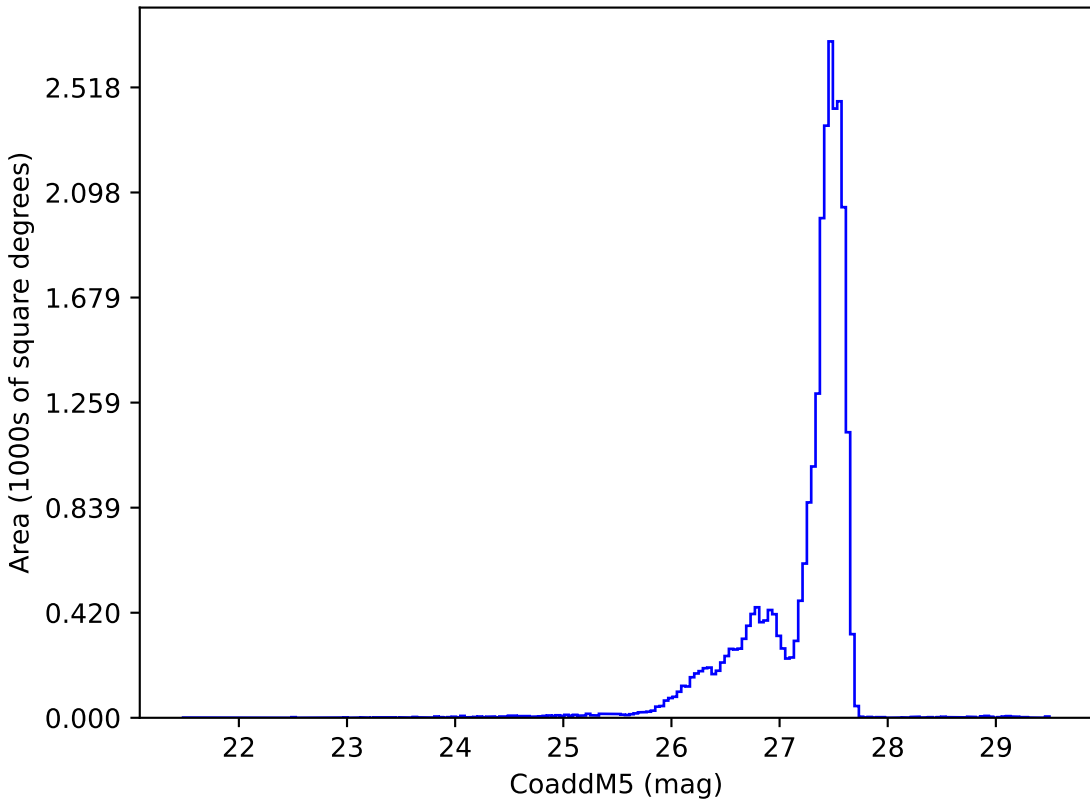
too_elab_r8_d2_gz_v3.4_10yrs : CoaddM5
