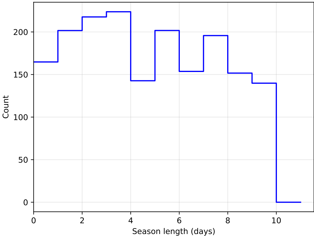
too_elab_r8_d2_gz_v3.4_10yrs DD:WFD all bands: SeasonLength
