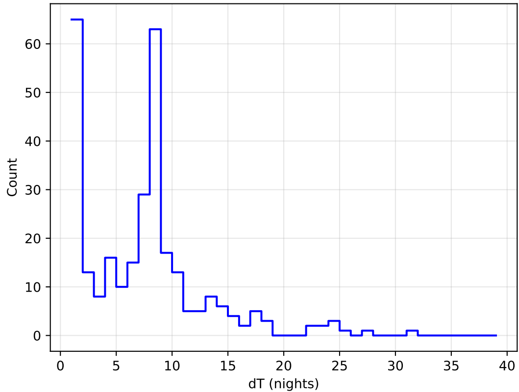
too_elab_r8_d2_gz_v3.4_10yrs all bands: DD:XMM_LSS Delta Nights Histogram
