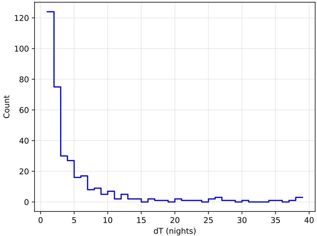
too_elab_r8_d2_gz_v3.4_10yrs all bands: DD:WFD Delta Nights Histogram
