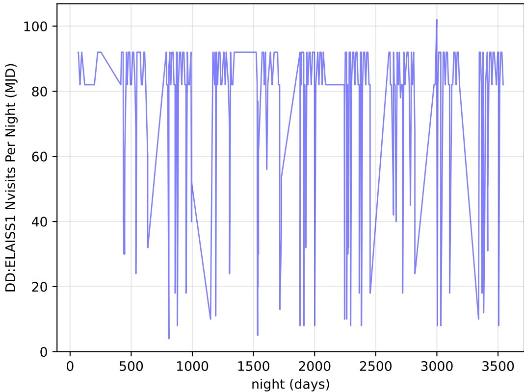
too_elab_r8_d2_gz_v3.4_10yrs all bands: DD:ELAISS1 Nvisits Per Night
