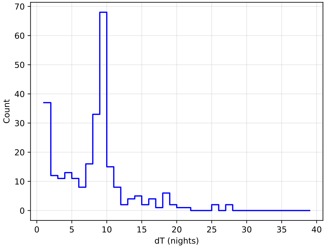
too_elab_r8_d2_gz_v3.4_10yrs all bands: DD:ELAISS1 Delta Nights Histogram
