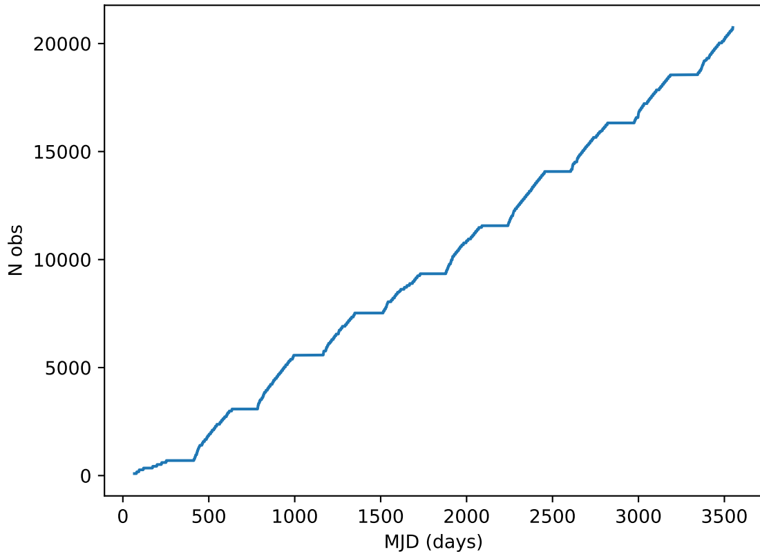
too_elab_r8_d2_gz_v3.4_10yrs all bands: DD:ELAISS1 Cumulative NVisits
