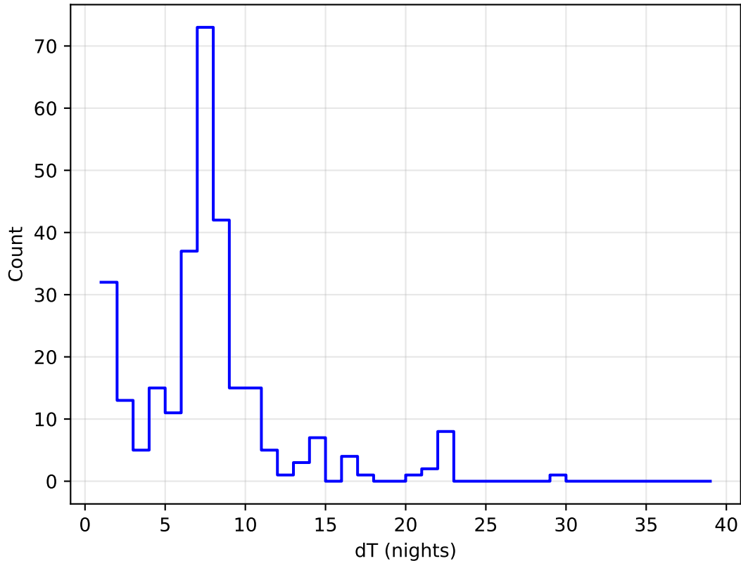
too_elab_r8_d2_gz_v3.4_10yrs all bands: DD:EDFS Delta Nights Histogram
