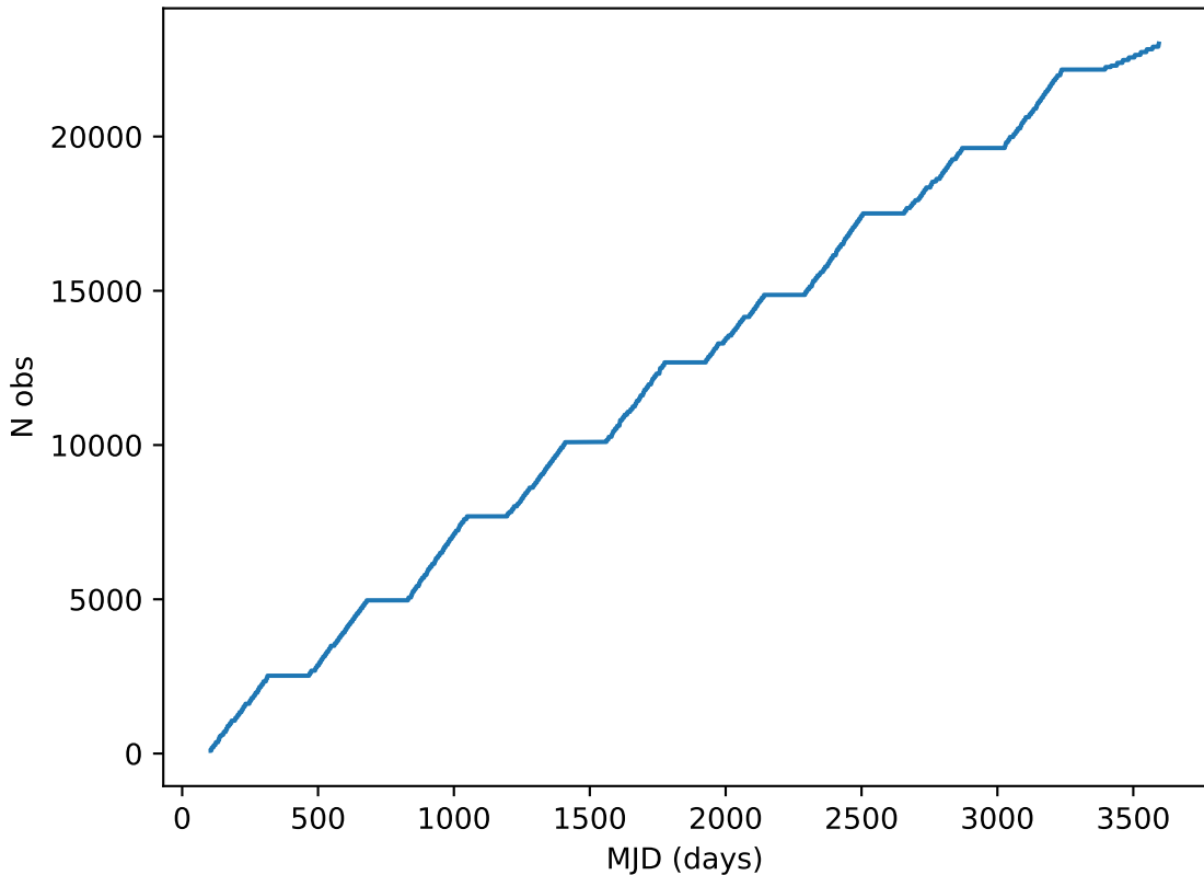
too_elab_r8_d2_gz_v3.4_10yrs all bands: DD:EDFS Cumulative NVisits
