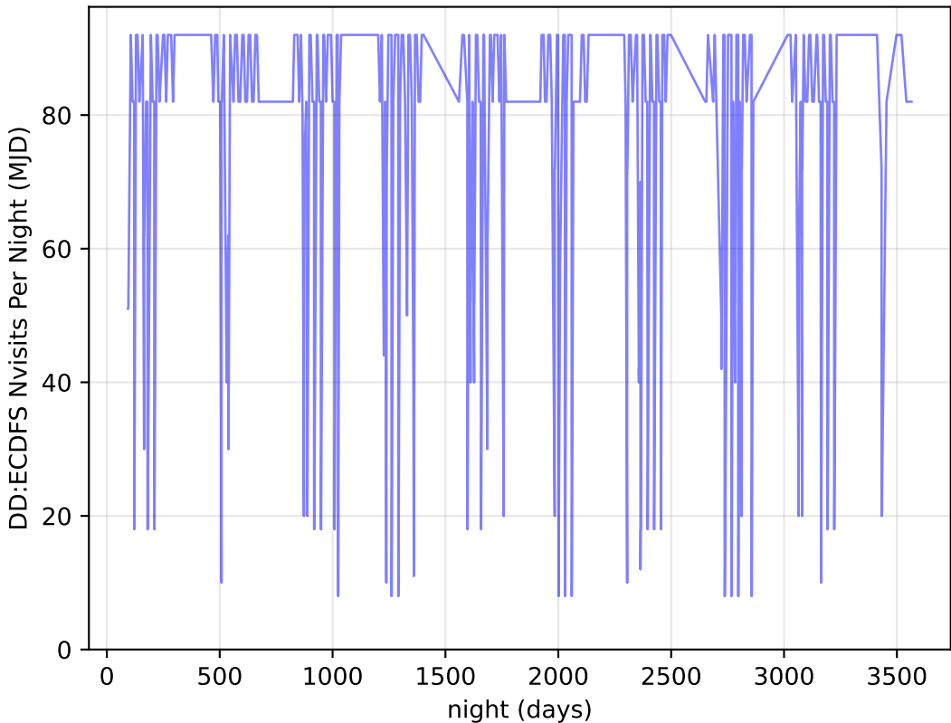
too_elab_r8_d2_gz_v3.4_10yrs all bands: DD:ECDFS Nvisits Per Night
