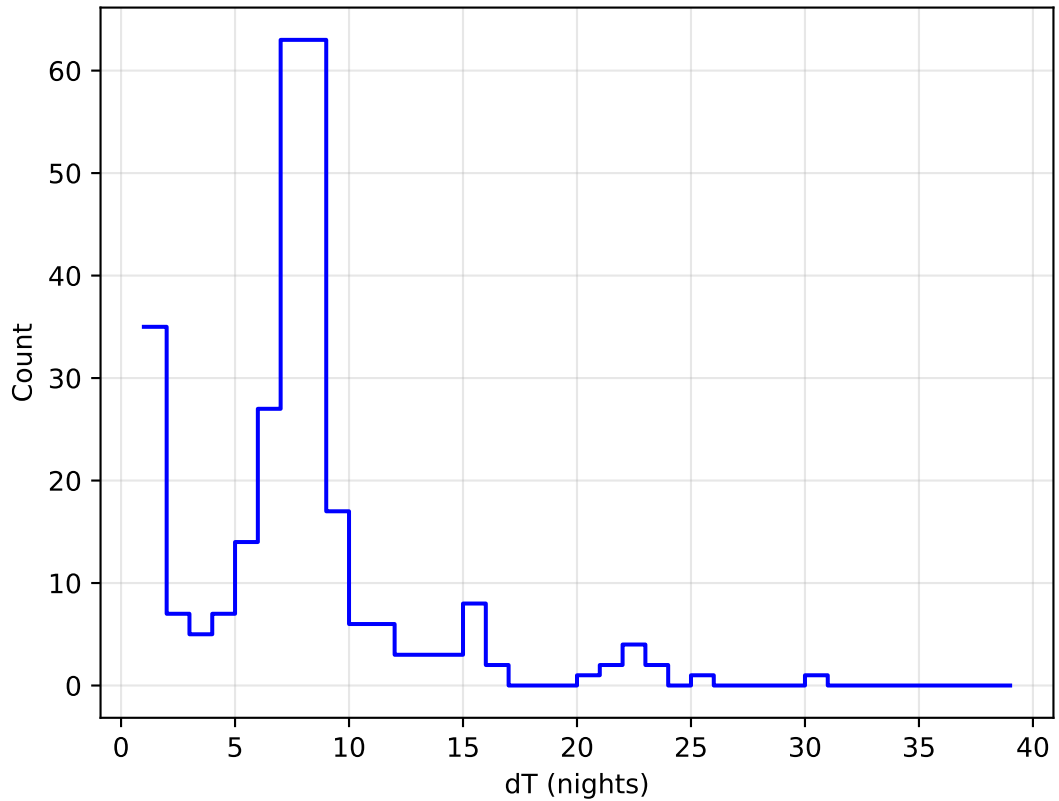
too_elab_r8_d2_gz_v3.4_10yrs all bands: DD:ECDFS Delta Nights Histogram
