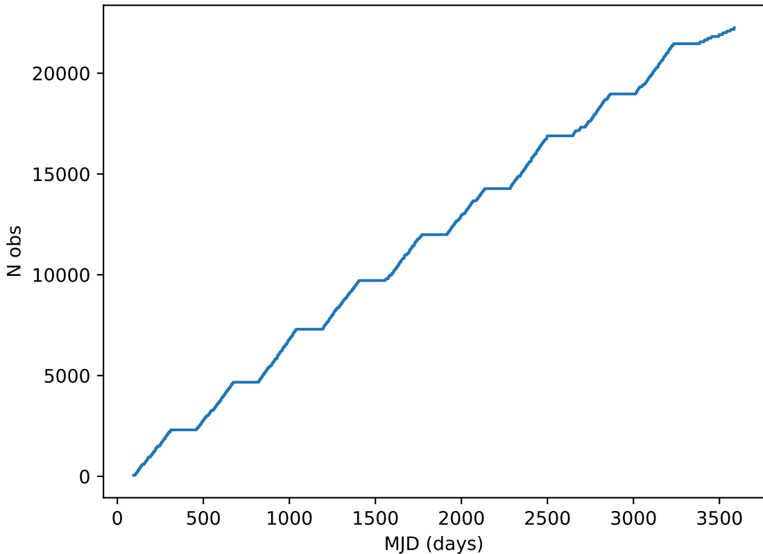
too_elab_r8_d2_gz_v3.4_10yrs all bands: DD:ECDFS Cumulative NVisits
