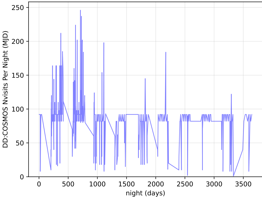
too_elab_r8_d2_gz_v3.4_10yrs all bands: DD: COSMOS Nvisits Per Night
