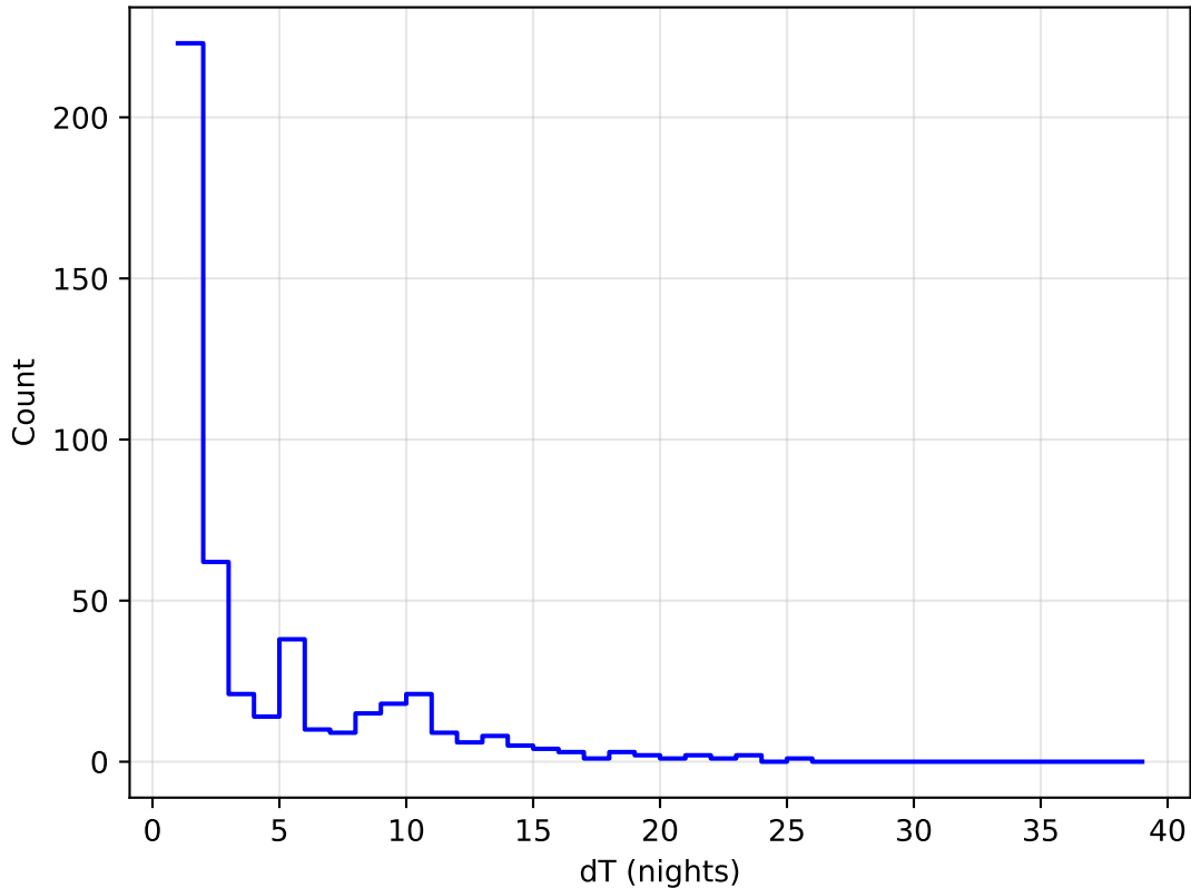
too_elab_r8_d2_gz_v3.4_10yrs all bands: DD: COSMOS Delta Nights Histogram
