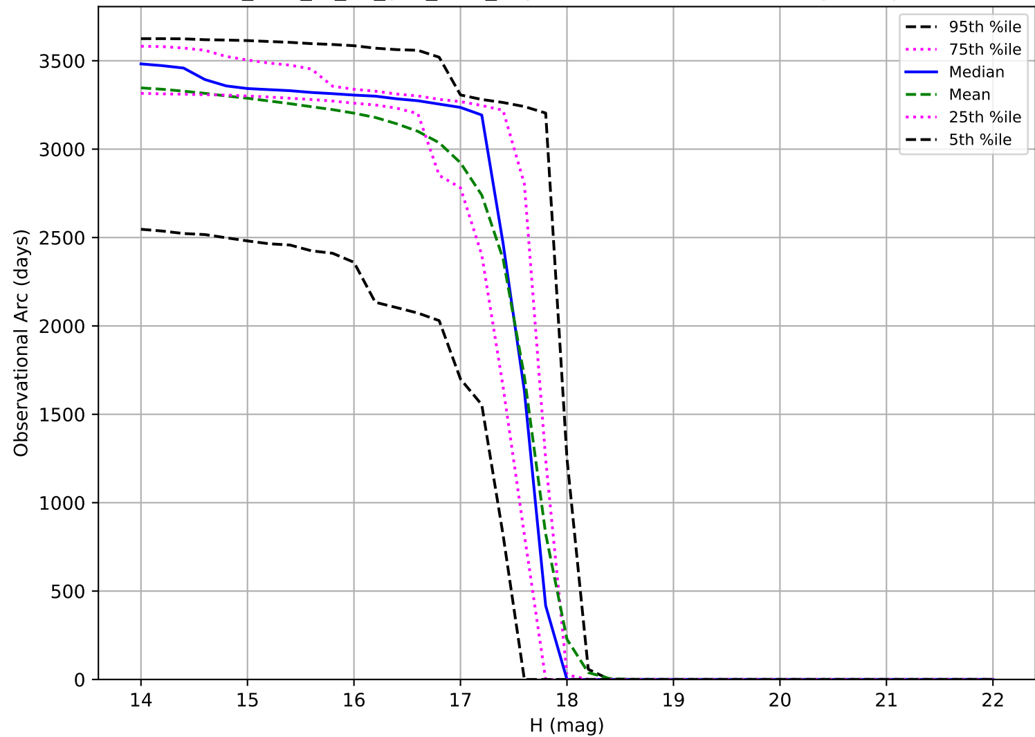
too_elab_r8_d2_griz_v3.4_10yrs: Observational Arc Length Trojan
