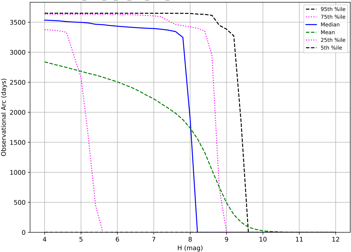
too_elab_r8_d2_griz_v3.4_10yrs: Observational Arc Length TNO
