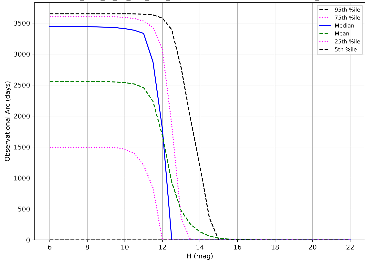
too_elab_r8_d2_griz_v3.4_10yrs: Observational Arc Length OCC_r20
