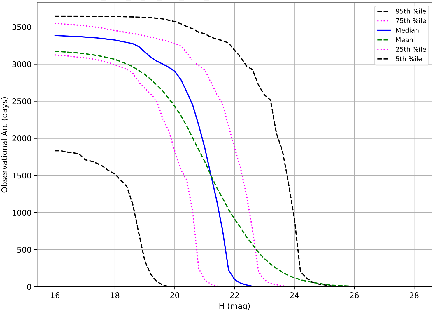
too_elab_r8_d2_griz_v3.4_10yrs: Observational Arc Length NEO
