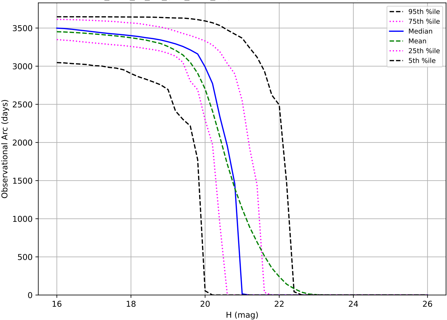
too_elab_r8_d2_griz_v3.4_10yrs: Observational Arc Length MBA
