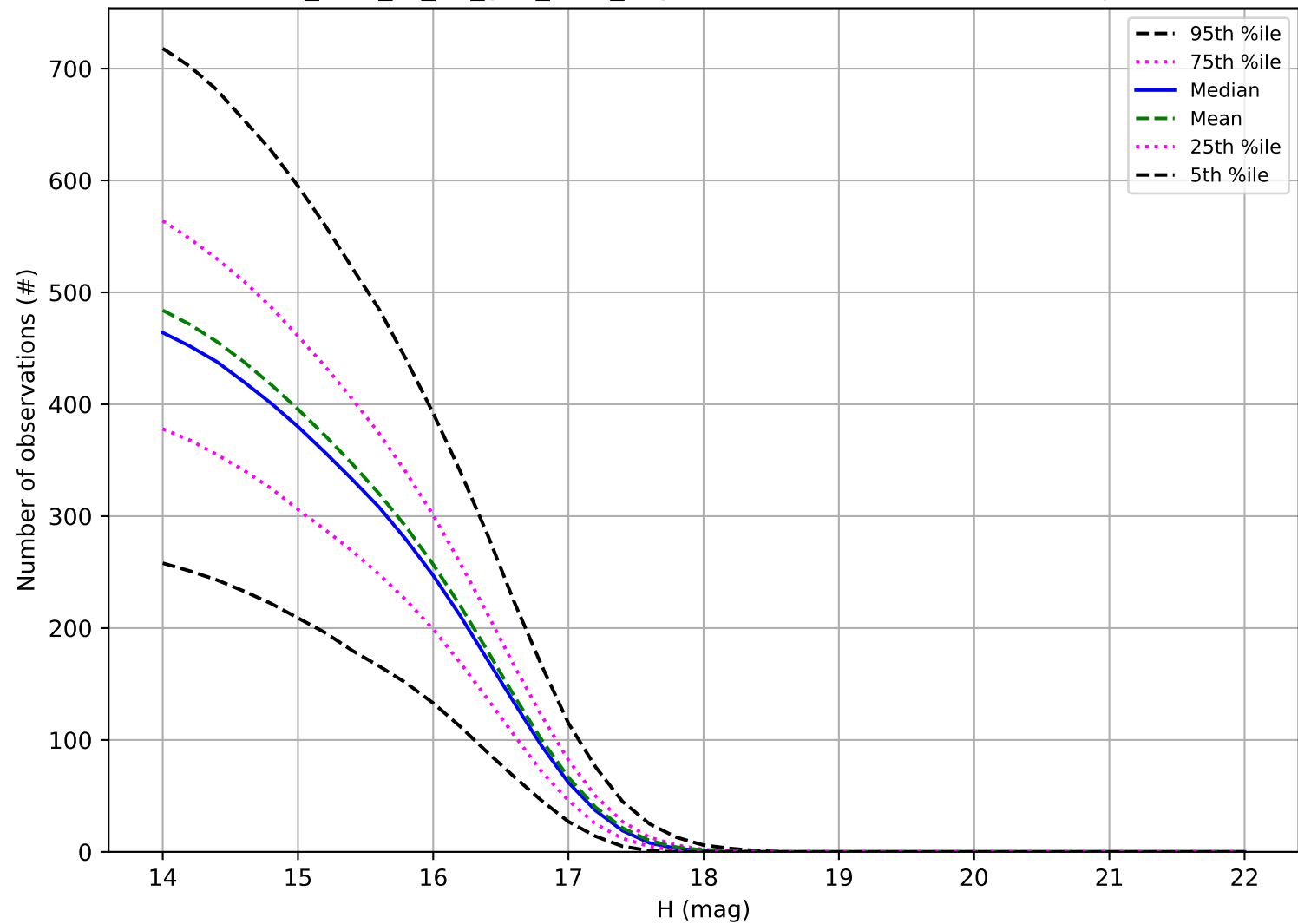
too_elab_r8_d2_griz_v3.4_10yrs: Number of observations Trojan
