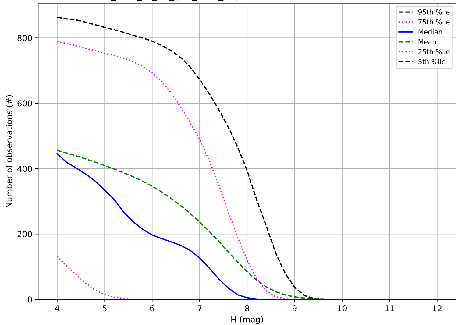
too_elab_r8_d2_griz_v3.4_10yrs: Number of observations TNO
