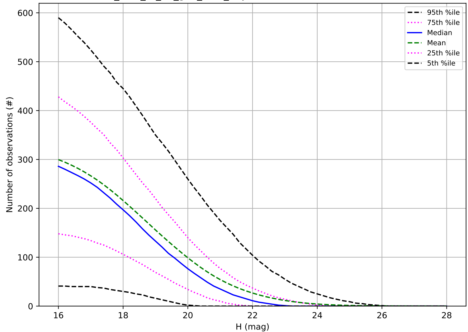
too_elab_r8_d2_griz_v3.4_10yrs: Number of observations PHA
