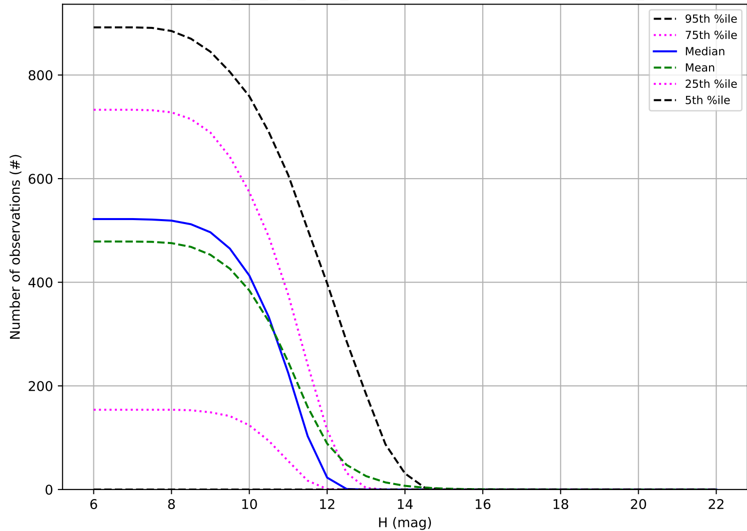
too_elab_r8_d2_griz_v3.4_10yrs: Number of observations OCC_r20
