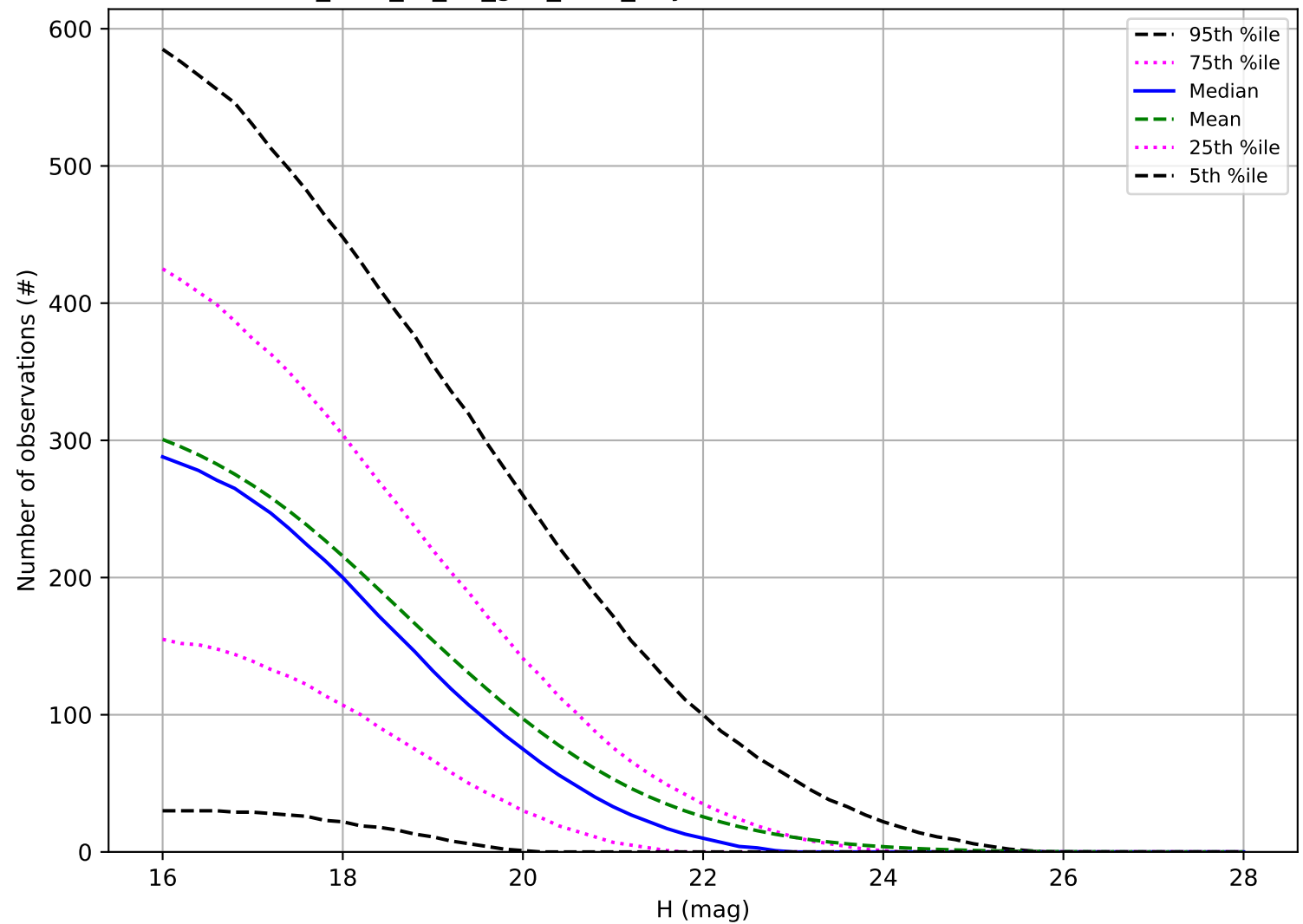
too_elab_r8_d2_griz_v3.4_10yrs: Number of observations NEO
