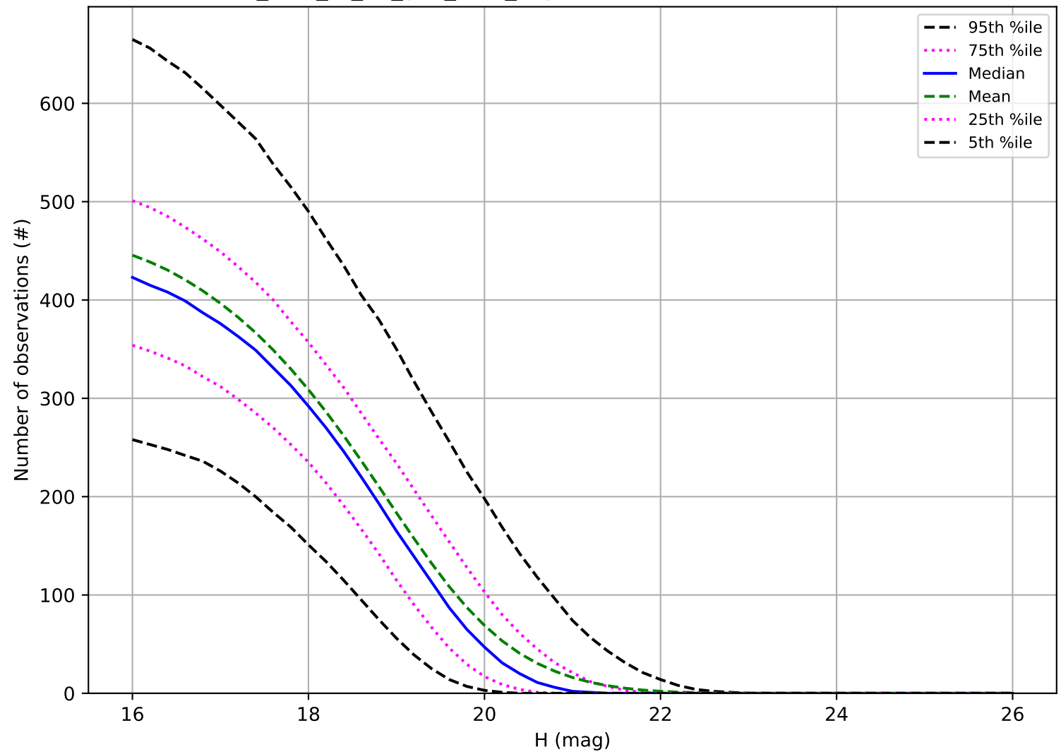
too_elab_r8_d2_griz_v3.4_10yrs: Number of observations MBA
