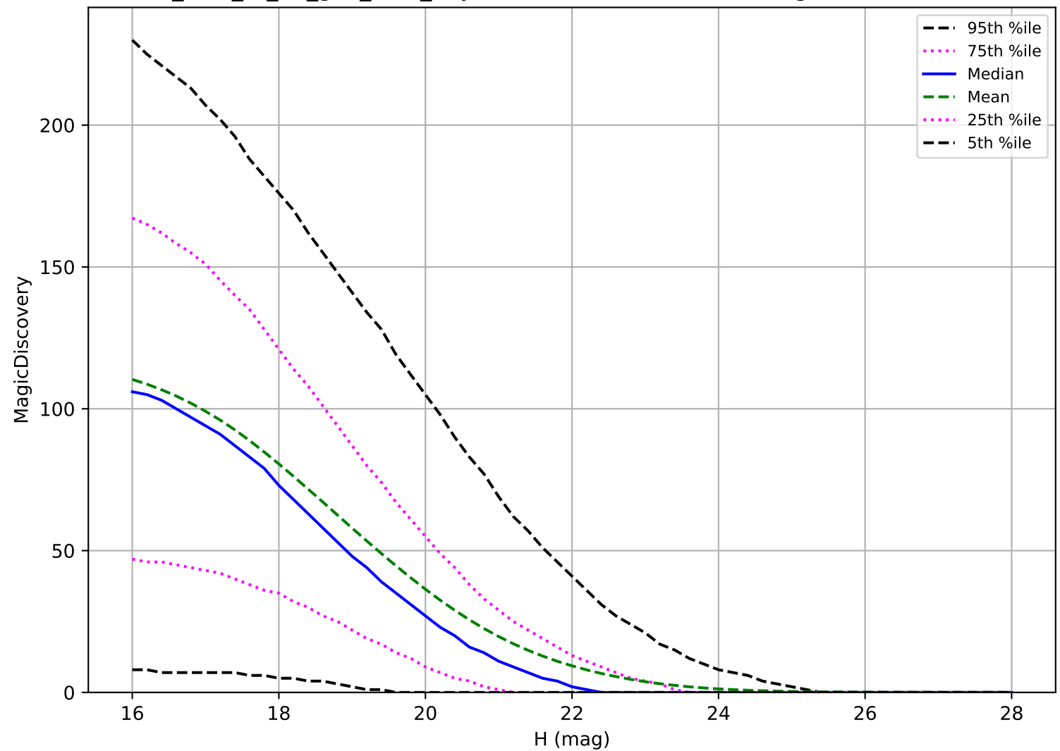
too_elab_r8_d2_griz_v3.4_10yrs: PHA 6 detections in 60 nights detection loss
