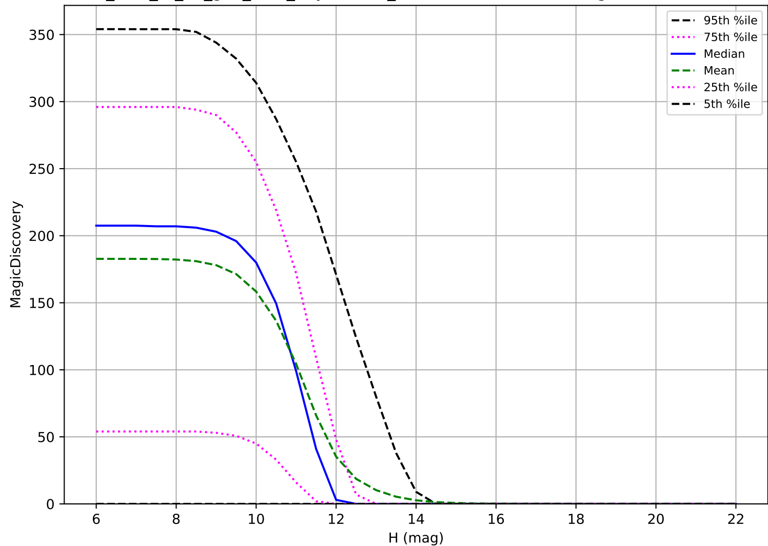
too_elab_r8_d2_griz_v3.4_10yrs: OCC_r20 6 detections in 60 nights detection loss
