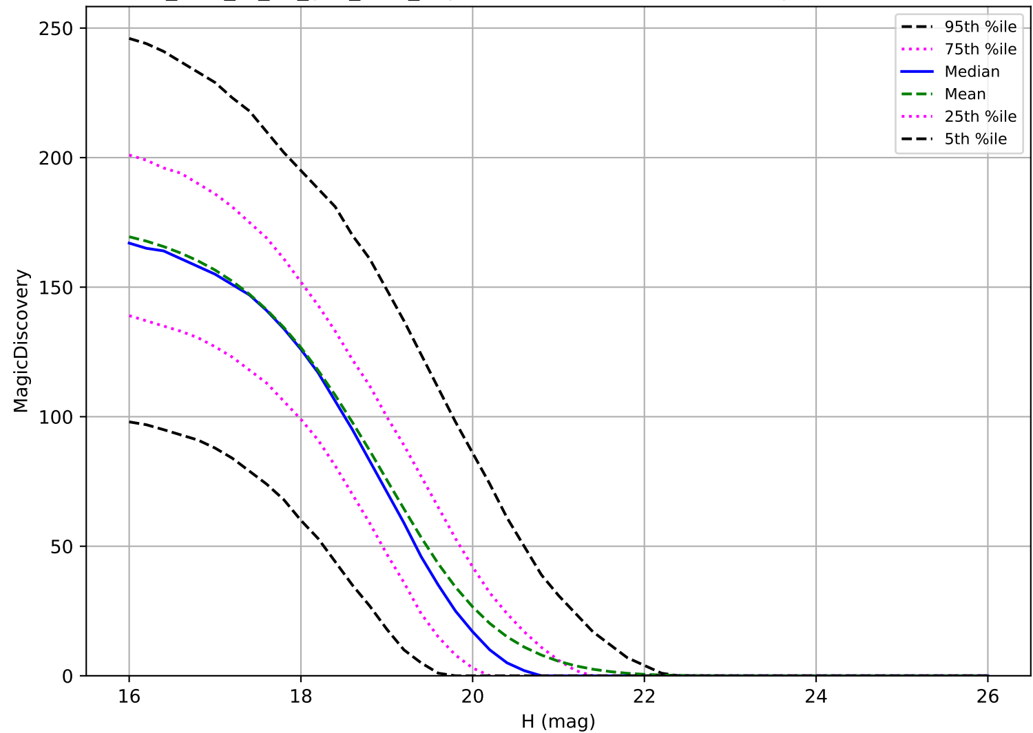
too_elab_r8_d2_griz_v3.4_10yrs: MBA 6 detections in 60 nights detection loss
