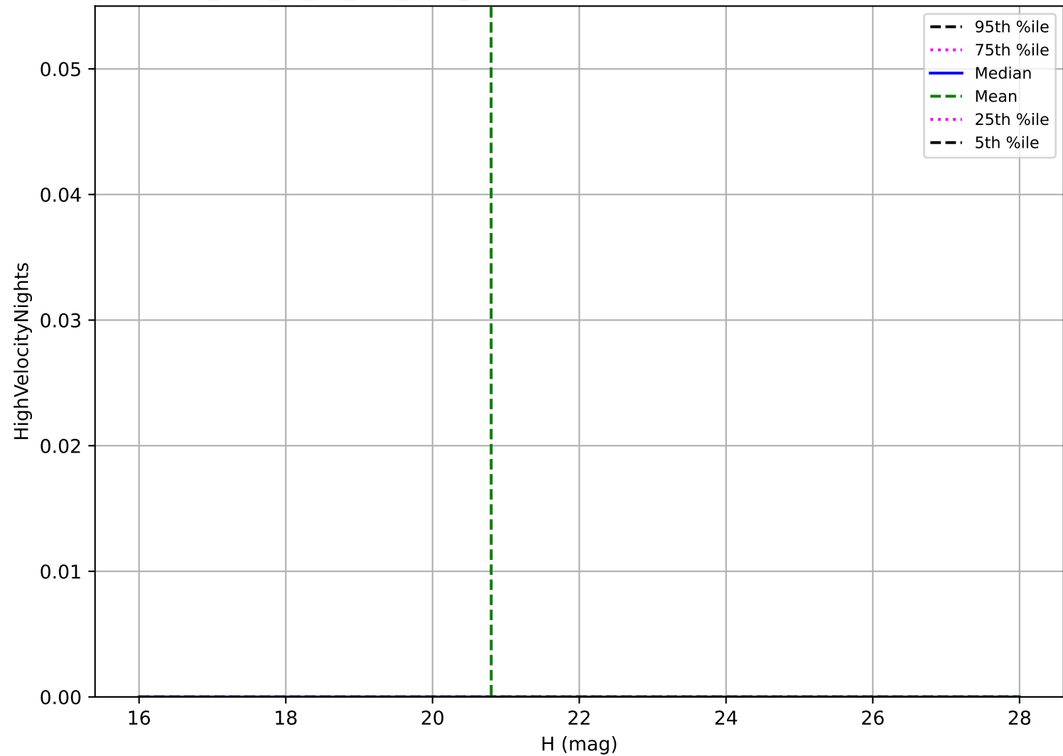
too_elab_r8_d2_griz_v3.4_10yrs: Vatira High velocity pair detection loss
