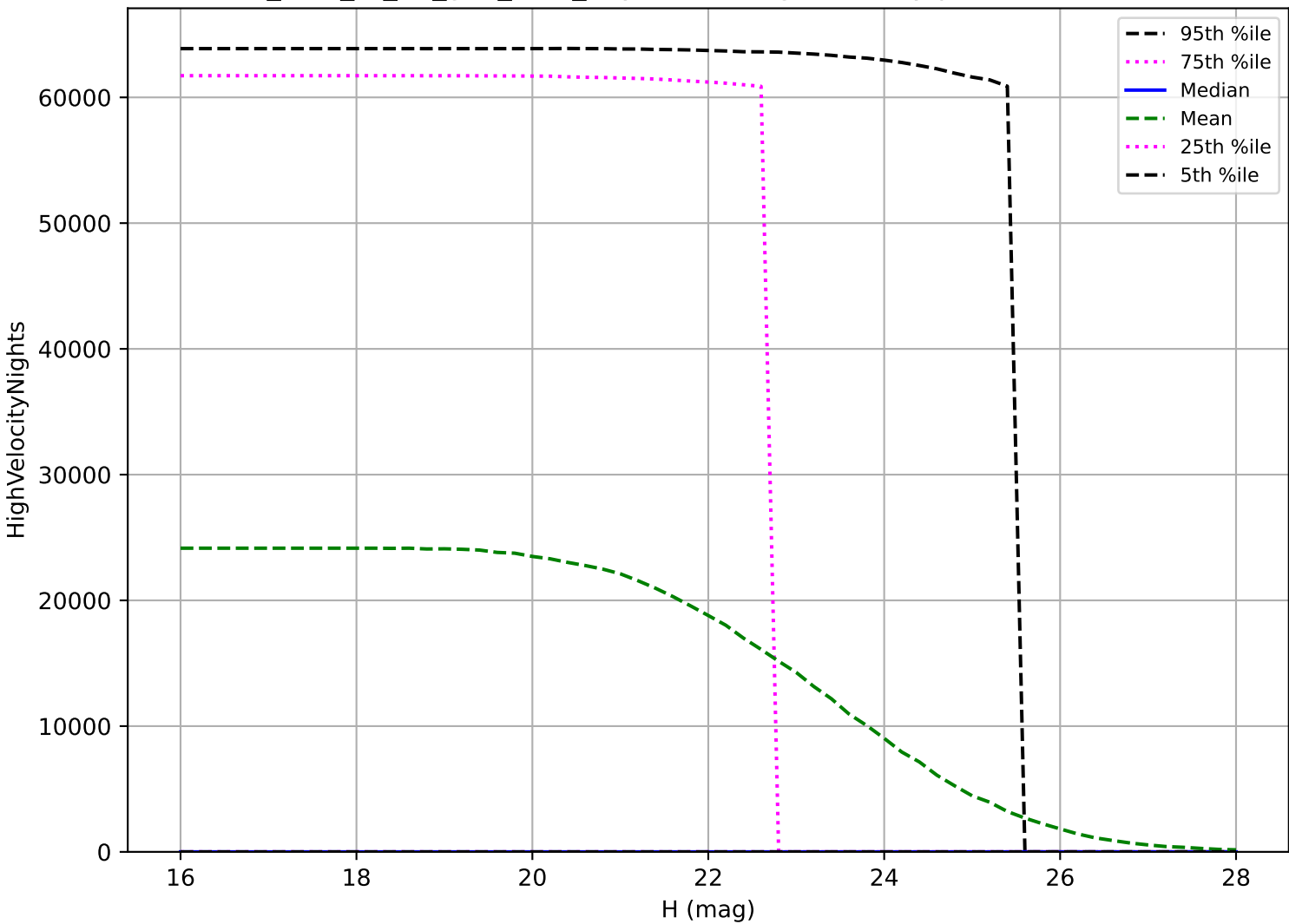
too_elab_r8_d2_griz_v3.4_10yrs: PHA High velocity pair detection loss
